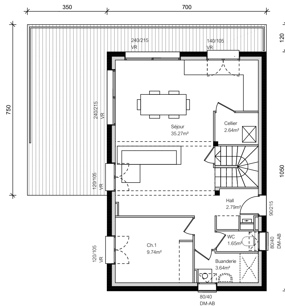
Plan Rez
